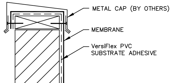
VersiFlex VFC-9B CAP FLASHING TERMINATION
